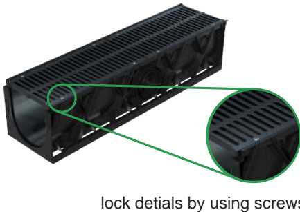
ID150/200/250/300/400/500 PP/HDPE Drain Channel And PP/HDPE Cover
