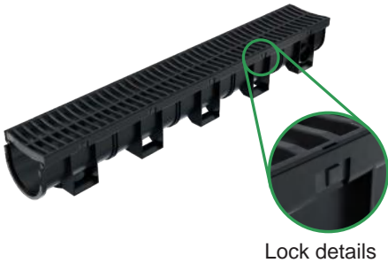
ID100 PP/HDPE Drain Channel And PP/HDPE Cover
