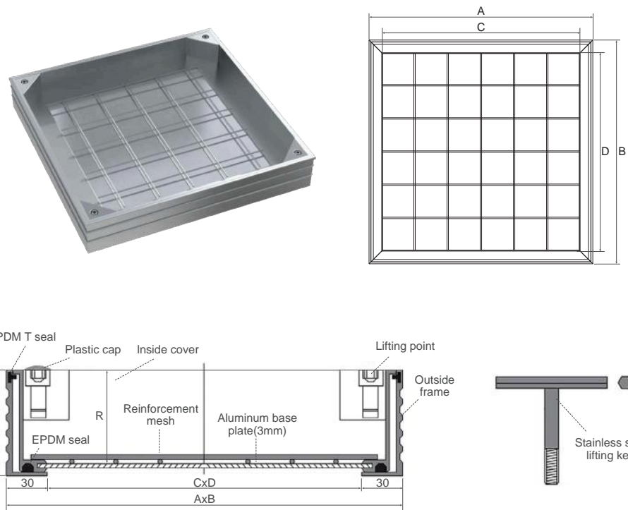
Aluminum manhole cover
