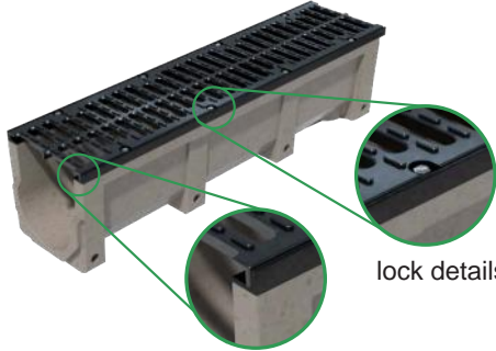
Polymer concrete drain channel and iron cast cover with side protect
