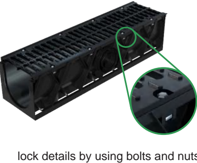
ID150/200/250/300/400/500 PP/HDPE Drain Channel And Iron cast cover
