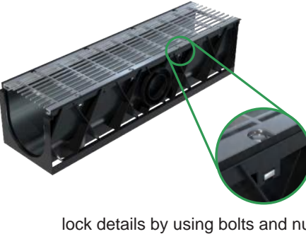
ID150/200/250/300/400/500 And galvanized steel mesh grate cover
