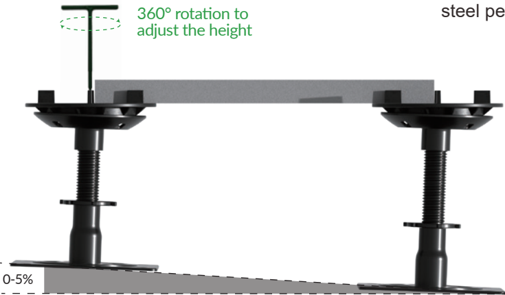
Self-leveling steel pedestal
