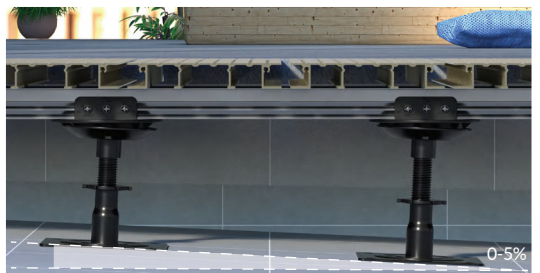
2. Slope compensation detail using self-leveling pedestal with aluminum joist and aluminum sheet.
