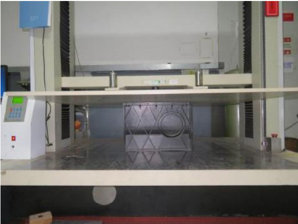
Fig.3 Pictures of sample during load-bearing test
