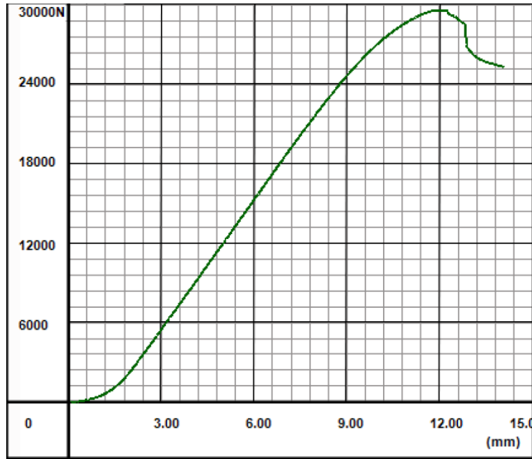
Fig.1 Test pressure curve picture of sample load-bearing test
